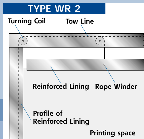
With type WR 2, the rope is laterally guided by an internal method.
